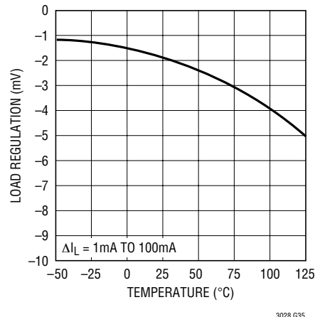
Output 2 Load Regulation
