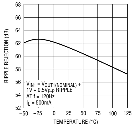
Output 1 Ripple Rejection
