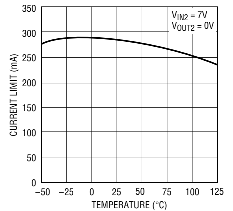
Output 2 Current Limit
