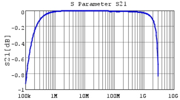
GR332DD72J333KW01 S21 DC0V,25degC
