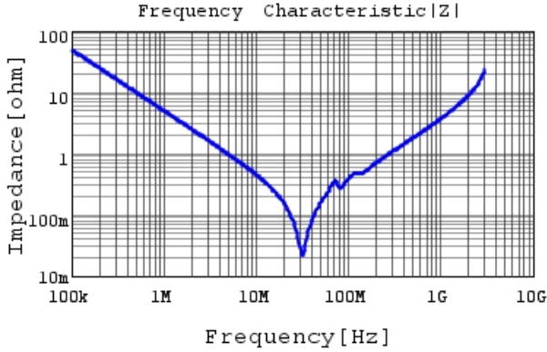
GR332DD72J333KW01 |Z| DCOV, 25degC
