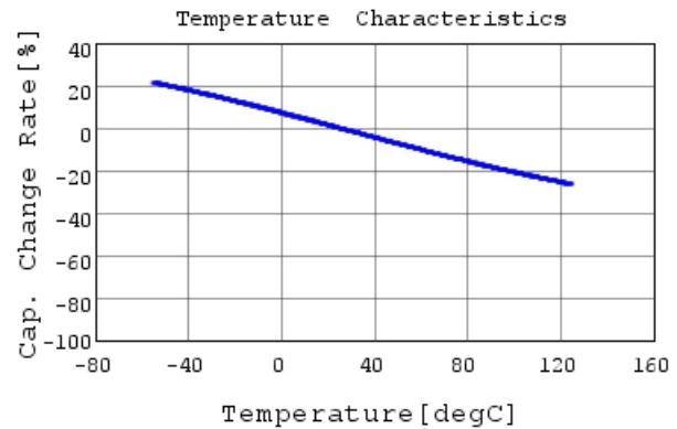
GR332DD72J333KW01 C-Temp. capchange, DCOV, 1
