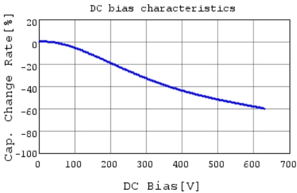
GR332DD72J333KW01 C-DC bias capchange, 25.0c
