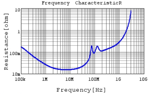
GR332DD72J333KW01 R DCOV, 25degC
