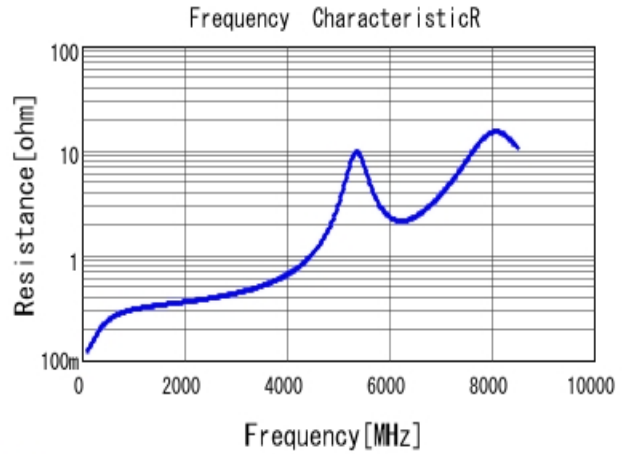
■ GRM1885C1H7R9BA01 R DCOV, 25degC
