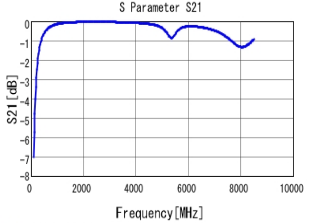
■ GRM1885C1H7R9BA01 S21 DCOV, 25degC
