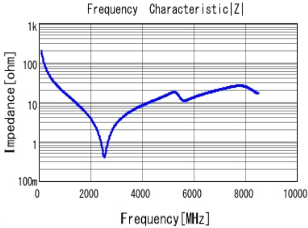
■ GRM1885C1H7R9BA01 |Z| DCOV, 25degC
