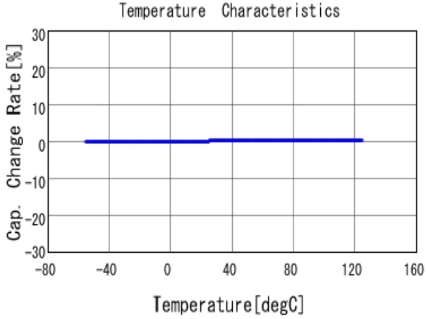
■ GRM1885C1H7R9BA01 C-Temp. capchange, DCOV, AC1Vrms
