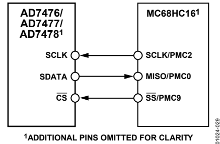
Figure 29. Interfacing to the MC68HC16
