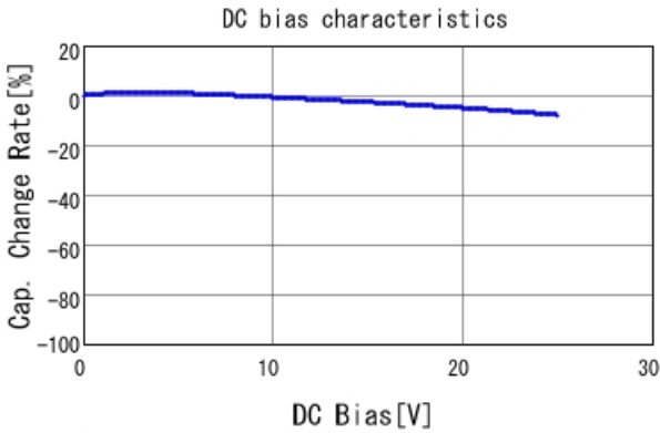
GCM188R71E103KA37 C-DC bias capchange, 25.0degC, A
