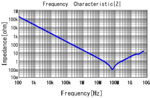
GCM188R71E103KA37 |Z| DCOV, 25degC
