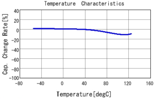
GCM188R71E103KA37 C-Temp. capchange, DC0.0V, AC1.C
