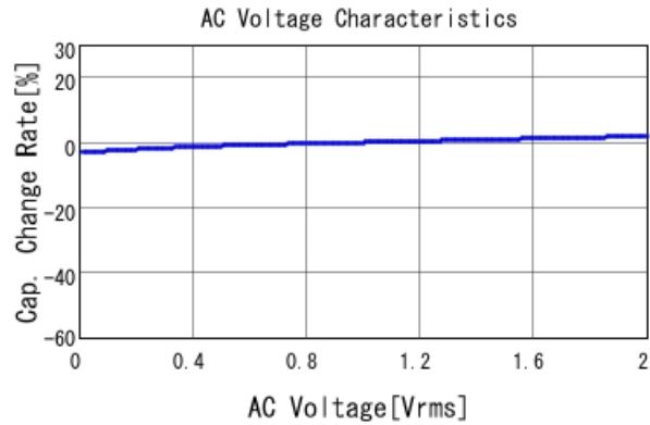
GCM188R71E103KA37 C-AC Voltage capchange, DCOV, 25
