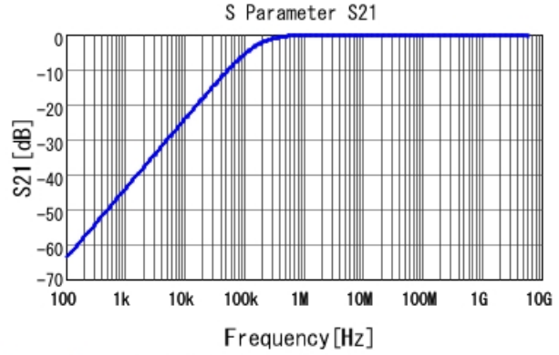
GCM188R71E103KA37 S21 DC0V, 25degC
