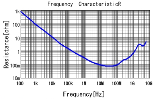
GCM188R71E103KA37 R DCOV, 25degC
