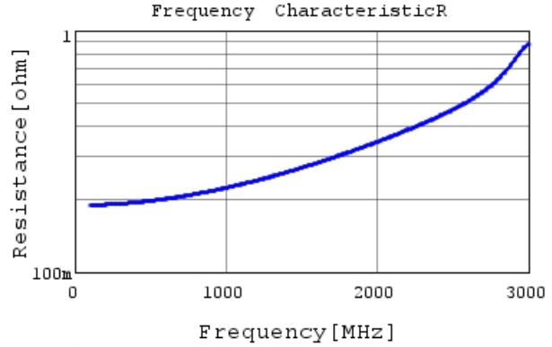
GRM31A5C3A100GW01 R DCOV, 25degC
