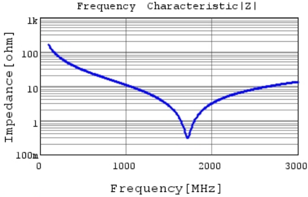
GRM31A5C3A100GW01 |Z| DCOV, 25degC
