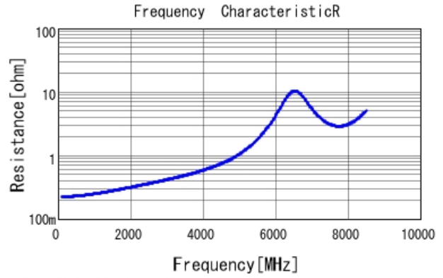
GCM1555C1H7R0BA16 R DC0V, 25degC
