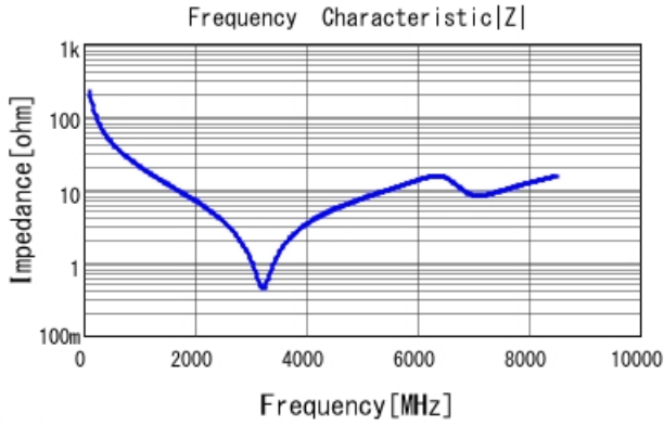
GCM1555C1H7R0BA16 |Z| DC0V, 25degC
