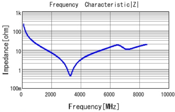
GRM1555C2A7R3BA01 |Z| DCOV, 25degC
