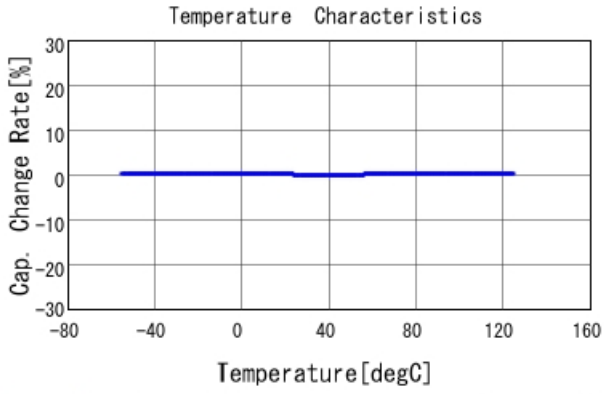
GRM1555C2A7R3BA01 C-Temp. capchange, DC0V, AC1Vrms
