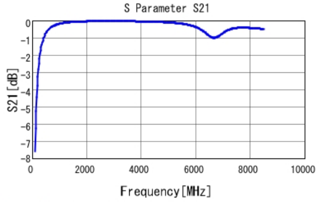
GRM1555C2A7R3BA01 S21 DC0V, 25degC
