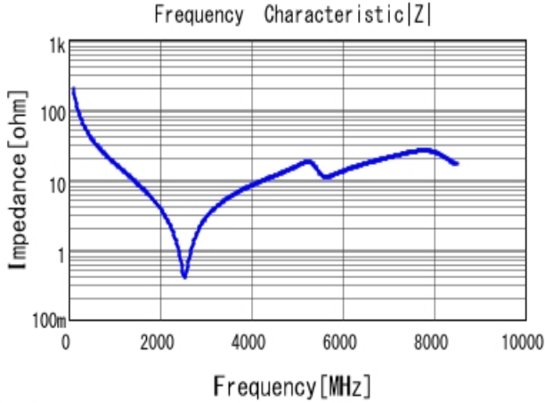
■ GRM1885C2A7R9BA01 |Z| DCOV, 25degC
