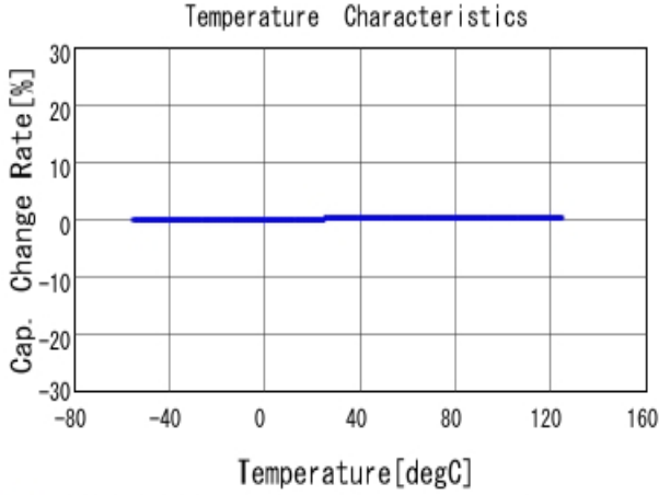
■ GRM1885C2A7R9BA01 C-Temp. capchange, DCOV, AC1Vrms
