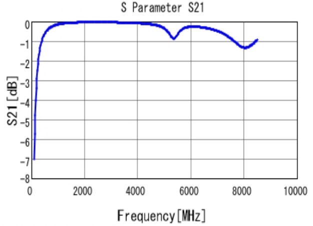
■ GRM1885C2A7R9BA01 S21 DCOV, 25degC
