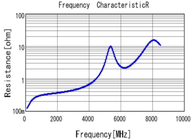
■ GRM1885C2A7R9BA01 R DCOV, 25degC
