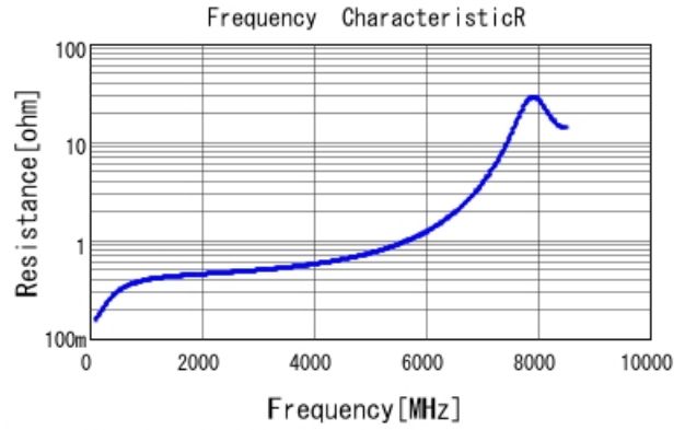
GRM1885C2A3R5WA01 R DCOV, 25degC
