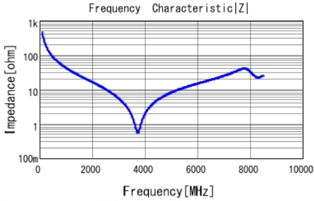
GRM1885C2A3R5WA01 |Z| DCOV, 25degC
