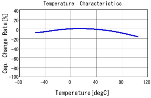
■ GRM188C81E475KE11 C-Temp. capchange, DCO. 0V, ACO. 5Vrm
