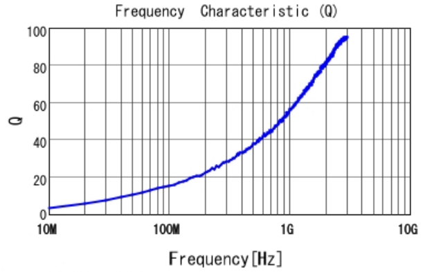
LQG15WH2N0B02 Q
