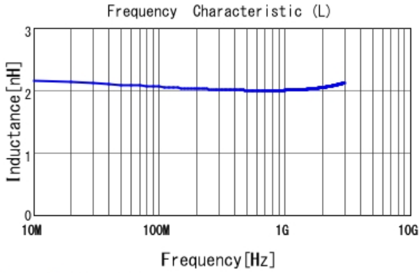
LQG15WH2N0B02 L
