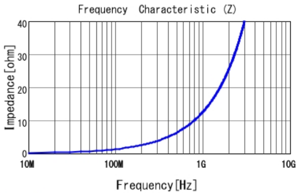
LQG15WH2N0B02 |Z|
