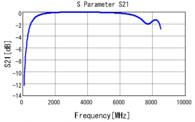
GRM1885C2A4R0BA01 S21 DC0V, 25degC
