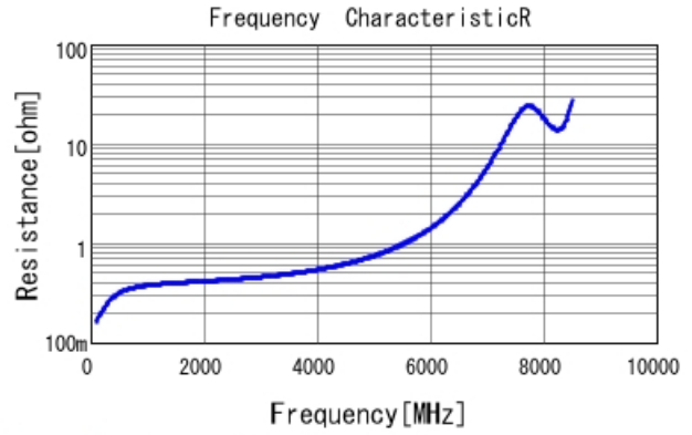
GRM1885C2A4R0BA01 R DCOV, 25degC
