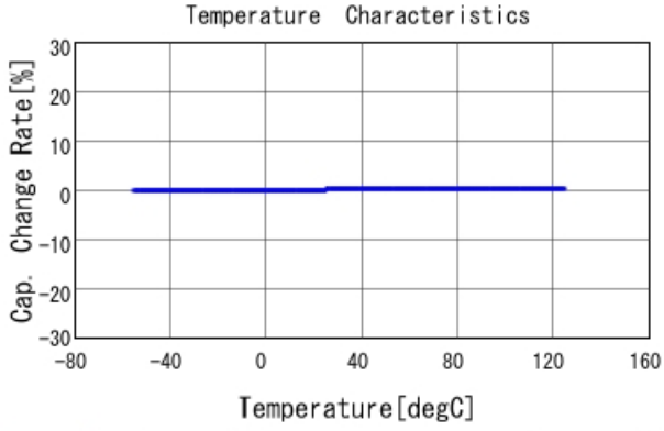
GRM1885C2A4R0BA01 C-Temp. capchange, DC0V, AC1Vrms
