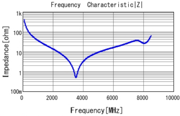
GRM1885C2A4R0BA01 |Z| DCOV, 25degC
