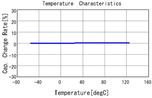
GJM1555C1H300FB01 C-Temp. capchange, DCOV, AC1Vrms
