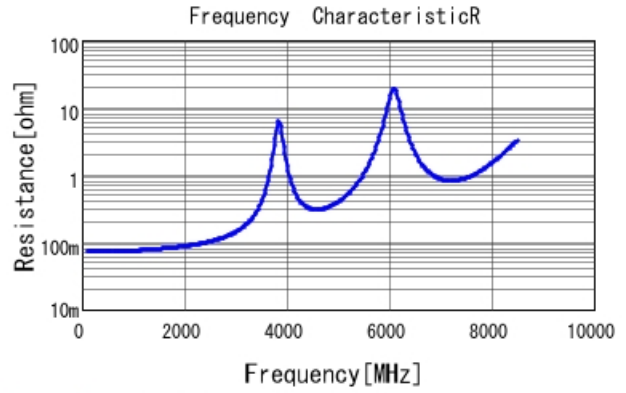
GJM1555C1H300FB01 R DCOV, 25degC
