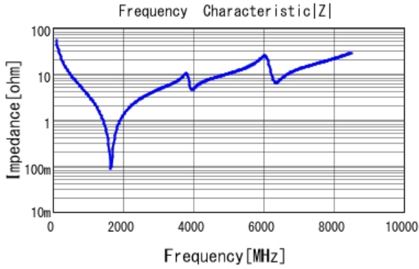
GJM1555C1H300FB01 |Z| DCOV, 25degC
