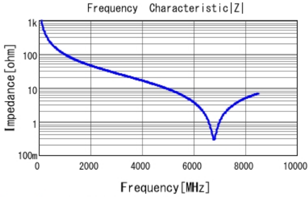
GJM1555C1H1R6CB01 |Z| DCOV, 25degC
