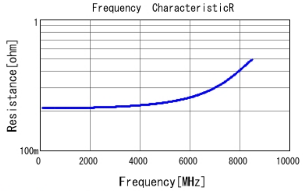
GJM1555C1H1R6CB01 R DCOV, 25degC
