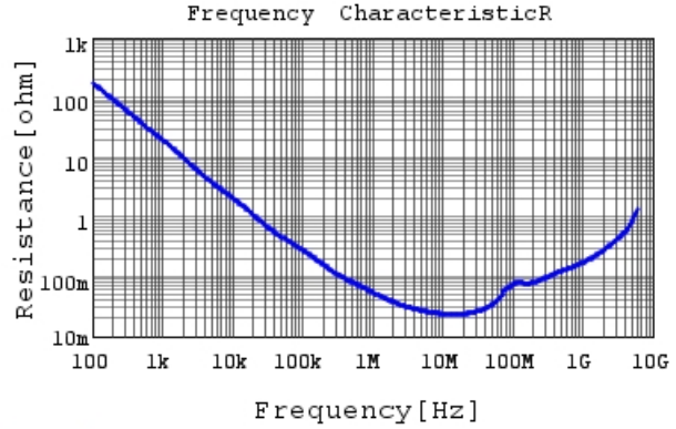
GRT155R71E473KE01 R DCOV,25degC
