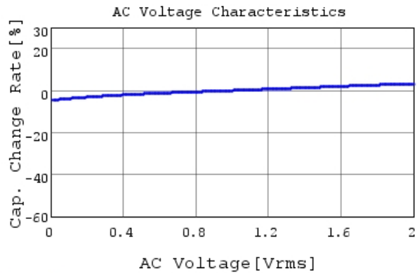
GRT155R71E473KE01 C-AC Voltage capchange, Dc
