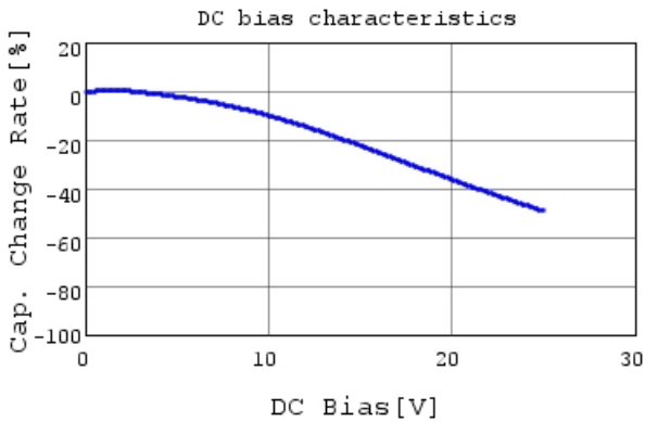
GRT155R71E473KE01 C-DC bias capchange, 25.0c
