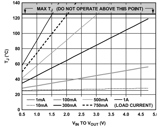
Figure 41. 0 mm 2 of PCB Copper, T A = 25°C, LFCSP
