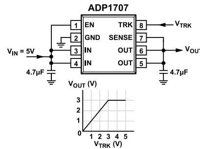
Figure 2. ADP1707 with Output Voltage Tracking
