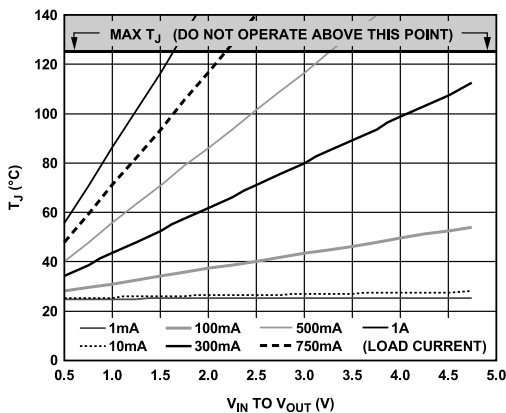
Figure 40. 100 mm 2 of PCB Copper, T A = 25°C, LFCSP
