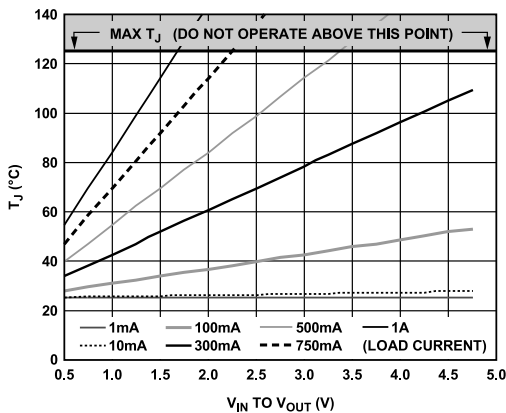
Figure 39. 500 mm 2 of PCB Copper, T A = 25°C, LFCSP
