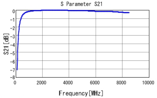
GRM1555C2A7R8WA01 S21 DCOV, 25degC
