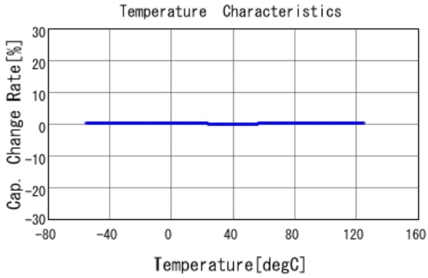
GRM1555C2A7R8WA01 C-Temp. capchange, DCOV, AC1Vrms
