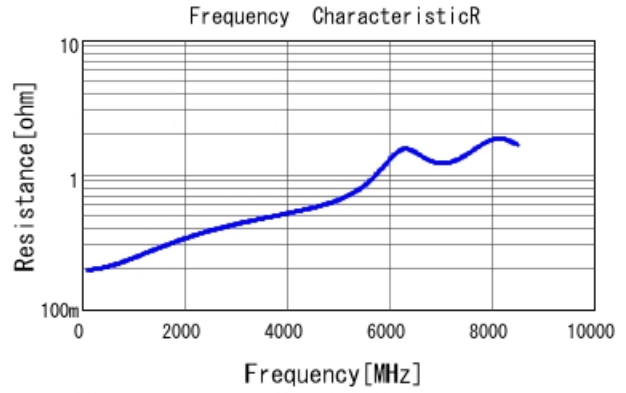
GRM1555C2A7R8WA01 R DCOV, 25degC
