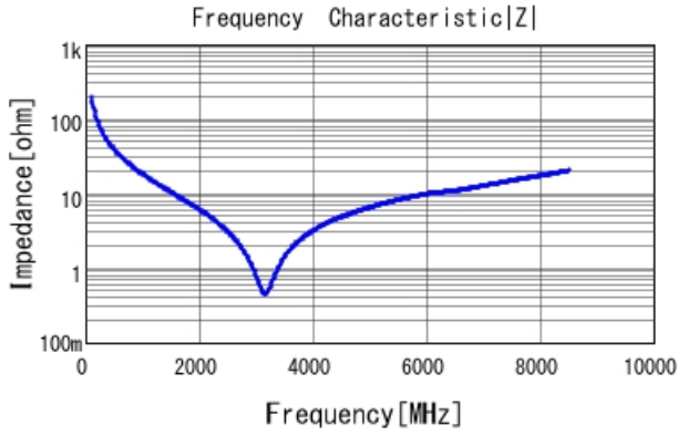
GRM1555C2A7R8WA01 |Z| DCOV, 25degC
