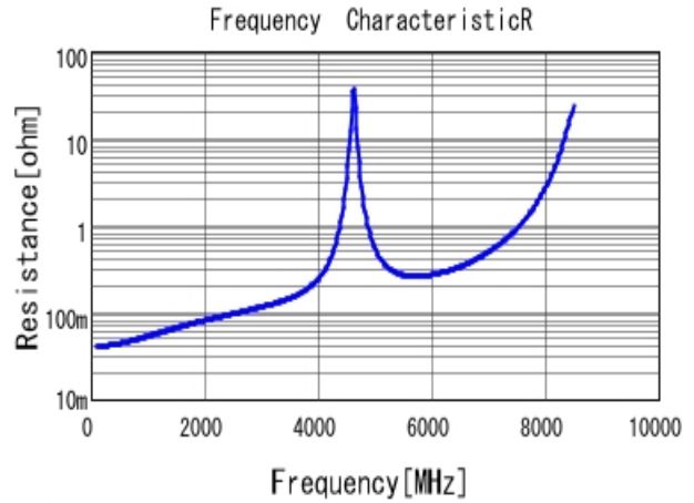
■ GQM2192C2A100JB01 R DC0V, 20degC
