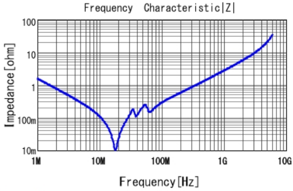
GRM3195C2A104JA01 |Z| DCOV, 25degC
