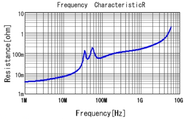
GRM3195C2A104JA01 R DCOV, 25degC
