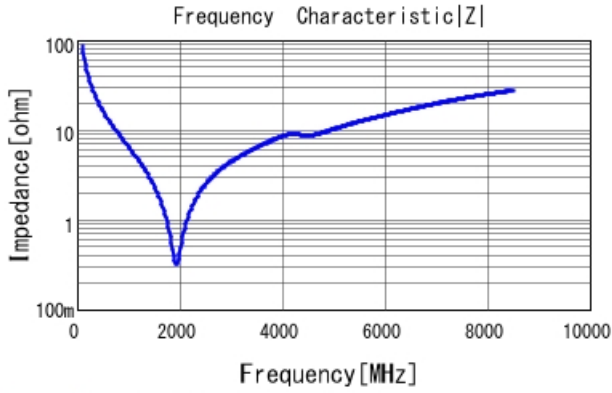
GRM1555C1H180GA01 |Z| DCOV, 25degC
