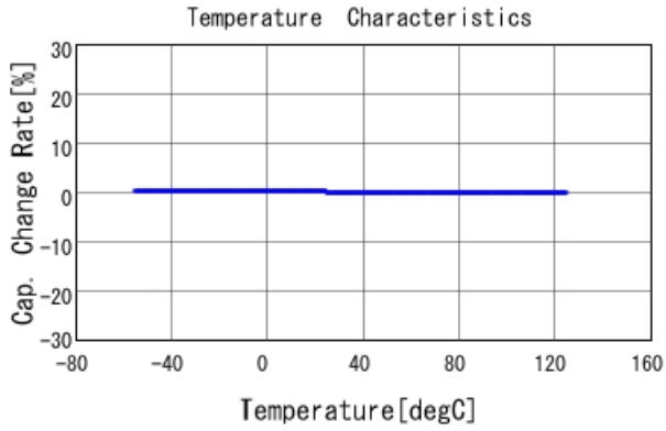
GRM1555C1H180GA01 C-Temp. capchange, DCOV, AC1Vrms
