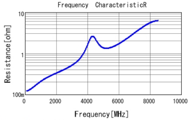
GRM1555C1H180GA01 R DCOV, 25degC
