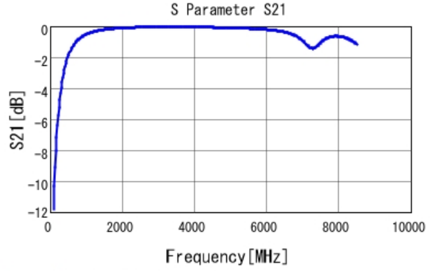
GRM1885C1H4R2BA01 S21 DCOV, 25degC
