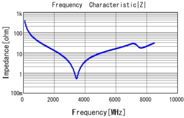
GRM1885C1H4R2BA01 |Z| DCOV, 25degC
