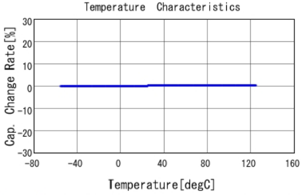
GRM1885C1H4R2BA01 C-Temp. capchange, DCOV, AC1Vrms
