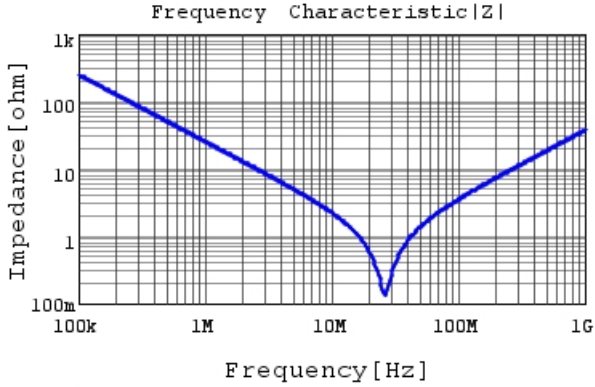
RDER72J682K2M1H03A |Z| DCOV, 25degC
