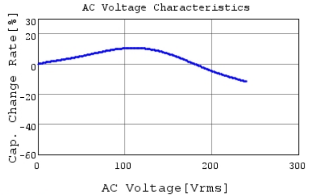
RDER72J682K2M1H03A C-AC Voltage capchange, I
