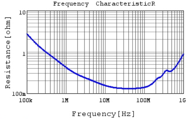
RDER72J682K2M1H03A R DCOV, 25degC
