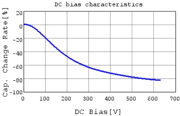
RDER72J682K2M1H03A C-DC bias capchange, 25.0
