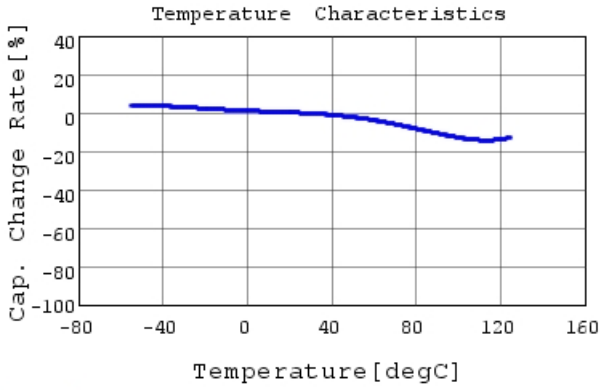
RDER72J682K2M1H03A C-Temp. capchange, DCOV,
