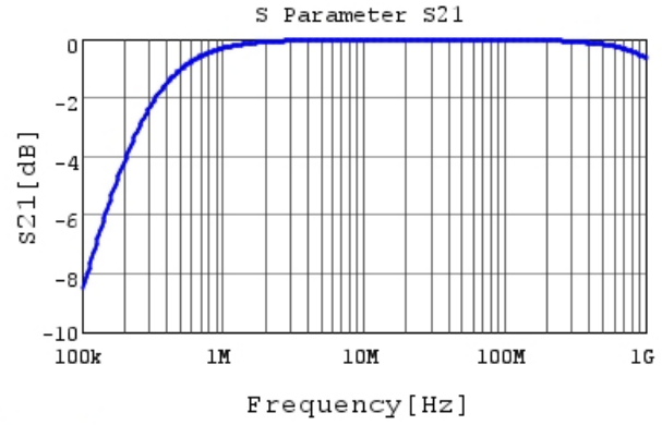
RDER72J682K2M1H03A S21 DCOV, 25degC
