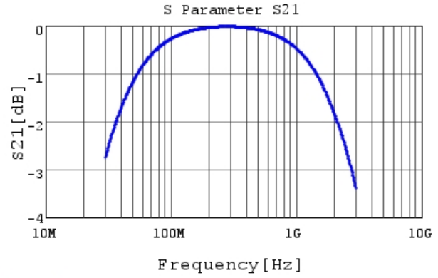
RDE5C1H560J0S1H03A S21 DCOV, 25degC
