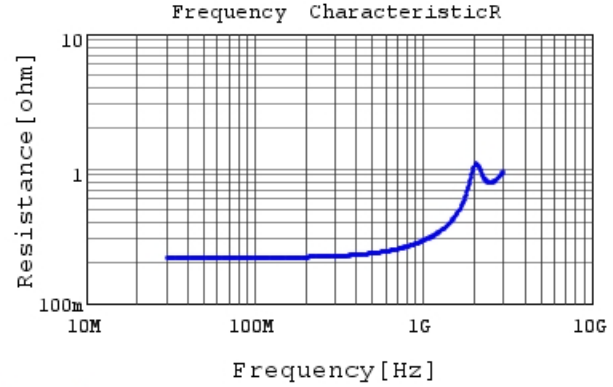
RDE5C1H560J0S1H03A R DC0V, 25degC
