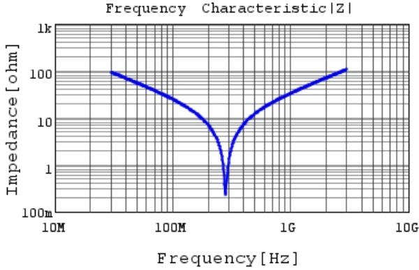
RDE5C1H560J0S1H03A |Z| DC0V, 25degC
