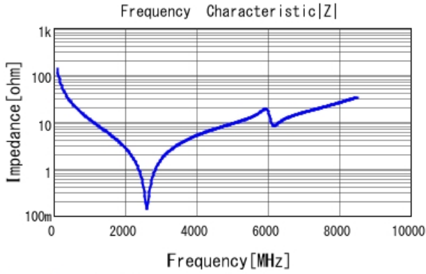
GJM1555C1H120JB01 |Z| DCOV, 25degC
