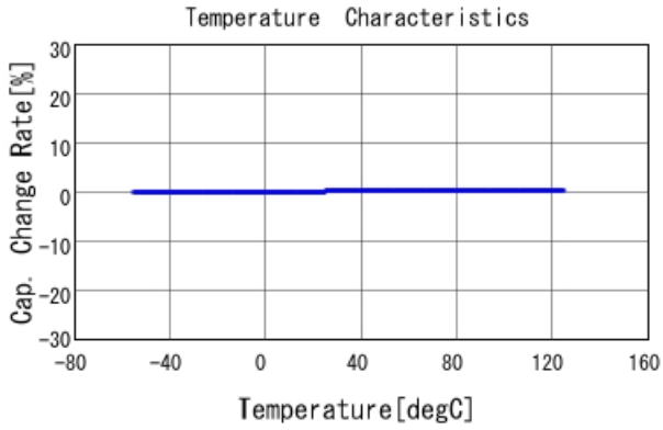
GJM1555C1H120JB01 C-Temp. capchange, DCOV, AC1Vrms
