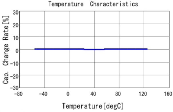
GRM1555C2A7R1CA01 C-Temp. capchange, DCOV, AC1Vrms
