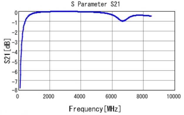
GRM1555C2A7R1CA01 S21 DCOV, 25degC
