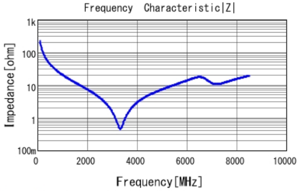
GRM1555C2A7R1CA01 |Z| DCOV, 25degC
