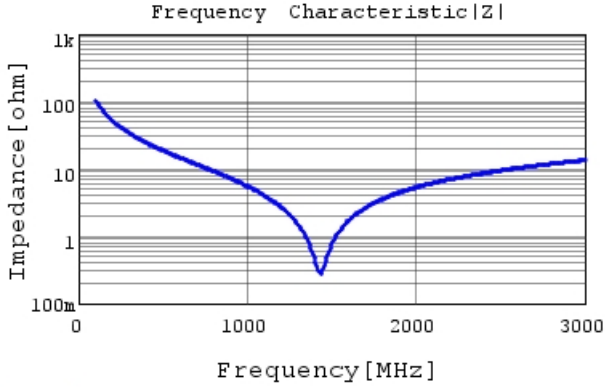
GRM31A5C2J150FW01 |Z| DCOV, 25degC
