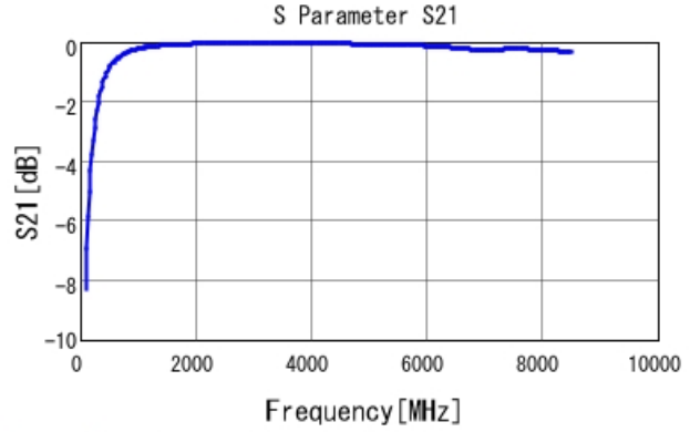
GRM1555C2A6R6DA01 S21 DCOV, 25degC
