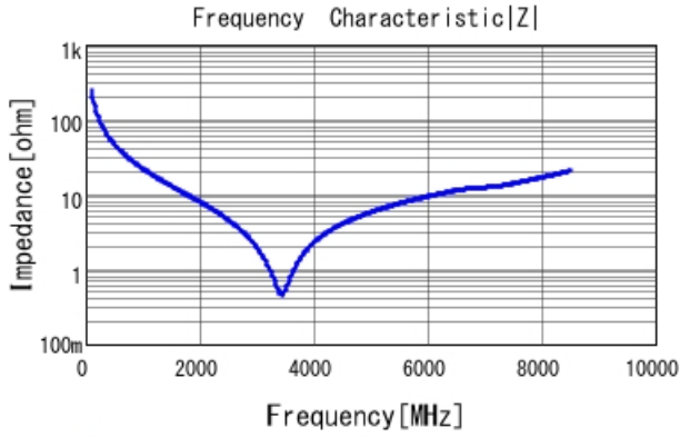
GRM1555C2A6R6DA01 |Z| DCOV, 25degC
