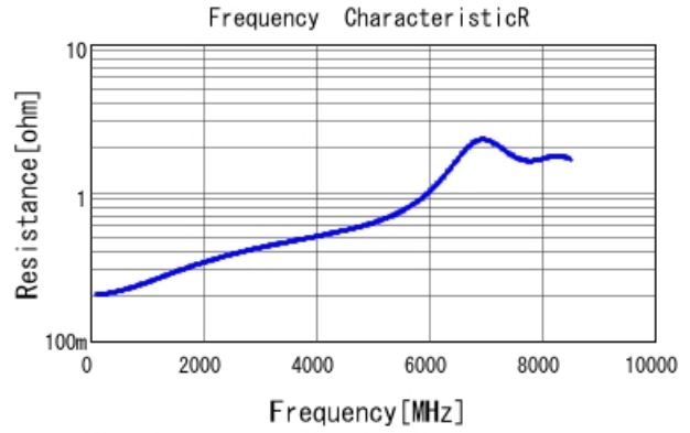
GRM1555C2A6R6DA01 R DCOV, 25degC
