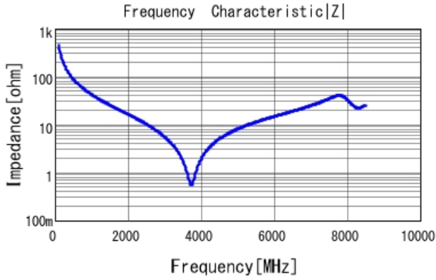
GRM1885C2A3R5CA01 |Z| DCOV, 25degC
