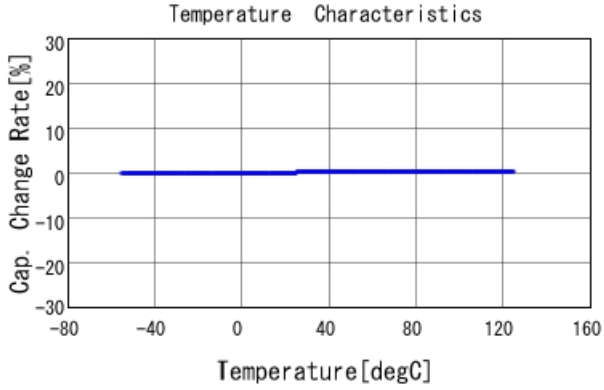
GRM1885C2A3R5CA01 C-Temp. capchange, DC0V, AC1Vrms
