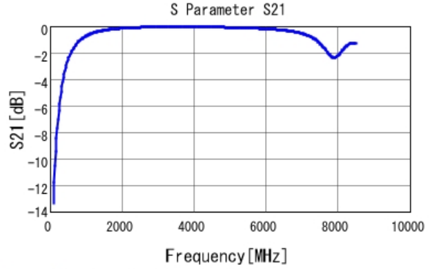
GRM1885C2A3R5CA01 S21 DC0V, 25degC
