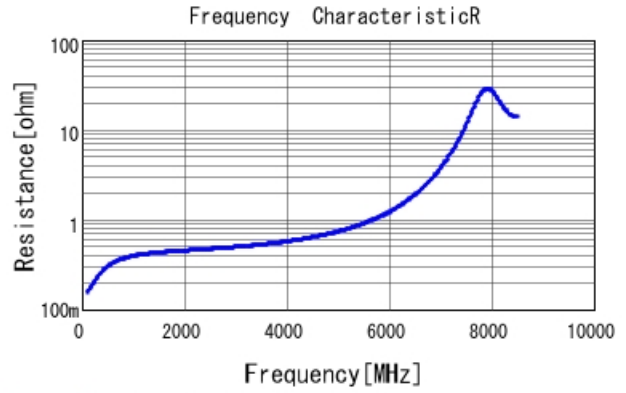
GRM1885C2A3R5CA01 R DCOV, 25degC
