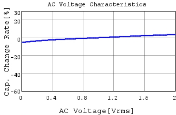
GRT155R71H104KE01 C-AC Voltage capchange, DC
