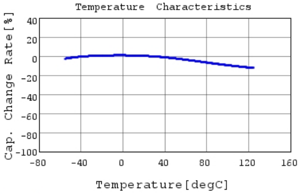
GRT155R71H104KE01 C-Temp. capchange, DC0.0V,
