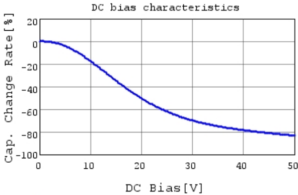
GRT155R71H104KE01 C-DC bias capchange, 25.0c
