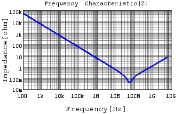
GRM033R61A333KE84 |Z| DCOV, 25degC
