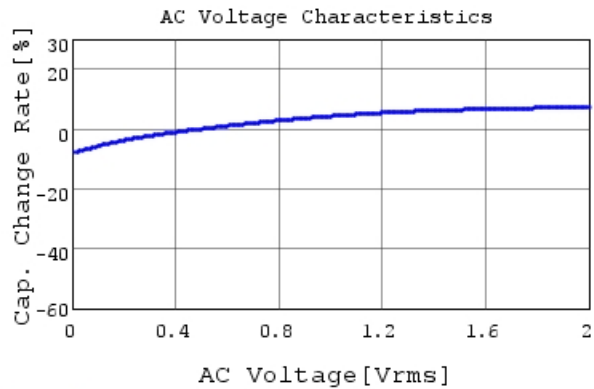
GRM033R61A333KE84 C-AC Voltage capchange, Dc
