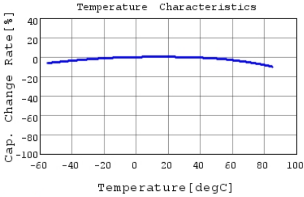
GRM033R61A333KE84 C-Temp. capchange, DC0.0V,
