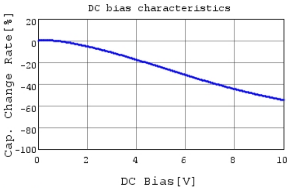
GRM033R61A333KE84 C-DC bias capchange, 25.0c
