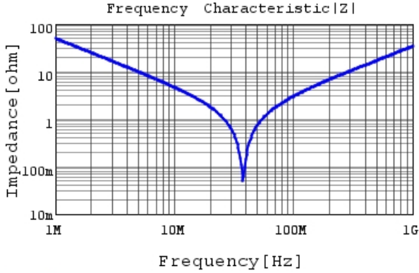
RDE5C1H332J0P1H03B |Z| DCOV, 25degC
