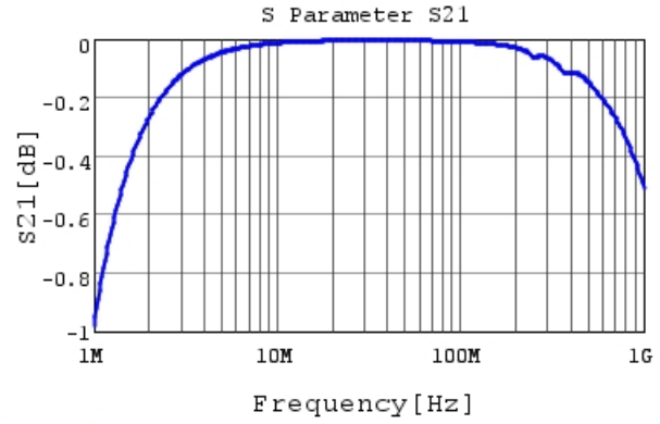
RDE5C1H332J0P1H03B S21 DCOV, 25degC
