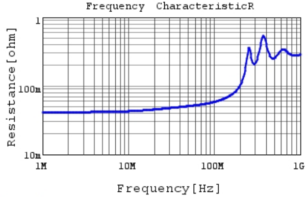
RDE5C1H332J0P1H03B R DCOV, 25degC
