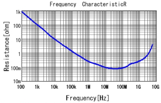
GRT155R71C103KE01 R DCOV, 25degC
