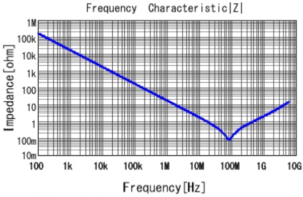
GRT155R71C103KE01 |Z| DCOV, 25degC
