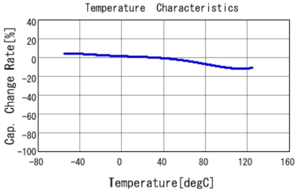
GRT155R71C103KE01 C-Temp. capchange, DC0.0V, AC1.C
