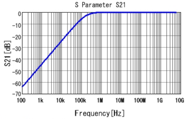
GRT155R71C103KE01 S21 DC0V, 25degC
