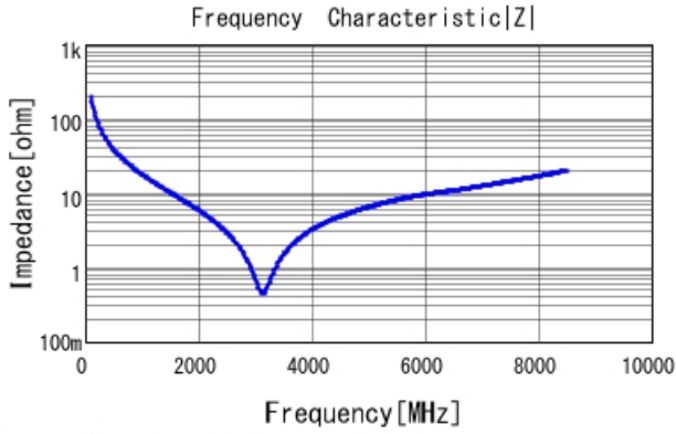
GRM1555C2A8R0WA01 |Z| DCOV, 25degC
