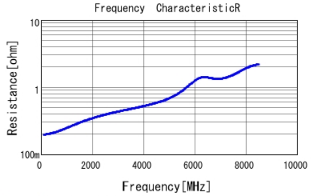
GRM1555C2A8R0WA01 R DCOV, 25degC
