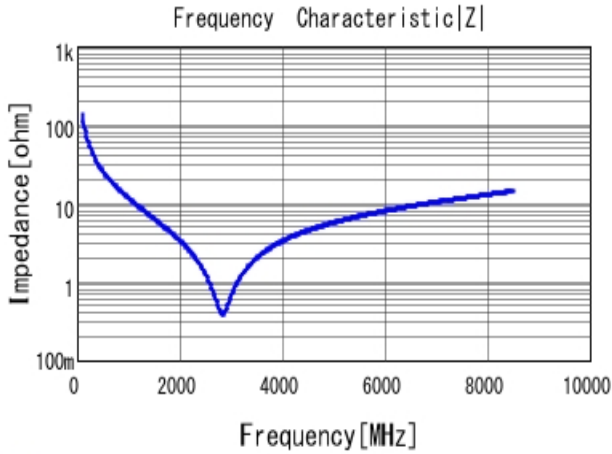
GCM0335C1E120GA16 |Z| DC0V, 25degC
