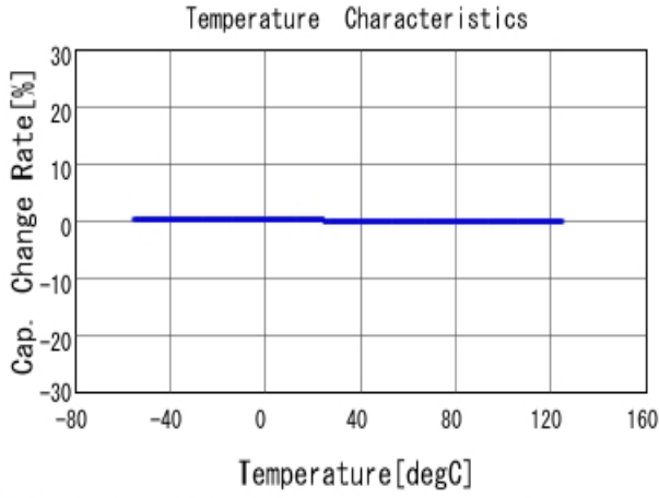
■ GCM0335C1E120GA16 C-Temp. capchange, DCOV, AC1Vrms
