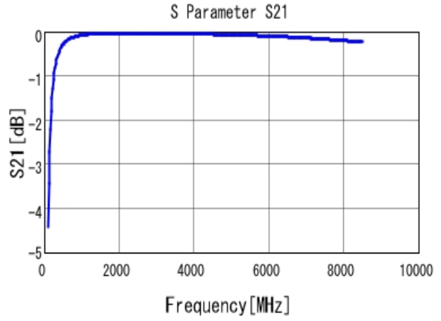
■ GCM0335C1E120GA16 S21 DCOV, 25degC
