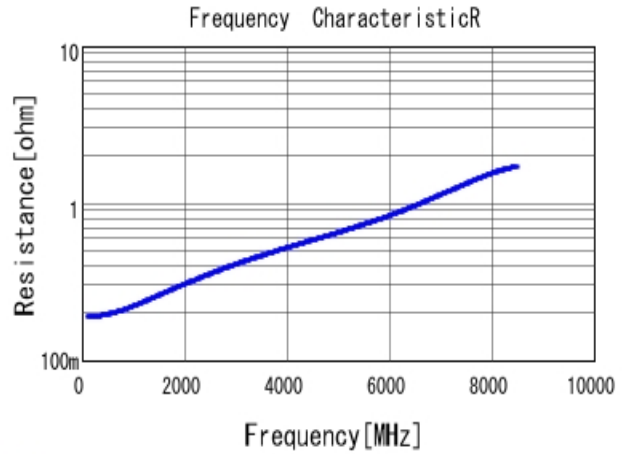
GCM0335C1E120GA16 R DC0V, 25degC
