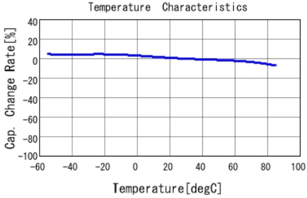
GRM219R61E106KA12 C-Temp. capchange, DC0.0V, AC1.C
