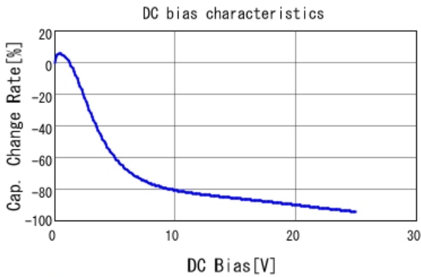
GRM219R61E106KA12 C-DC bias capchange, 25.0degC, A
