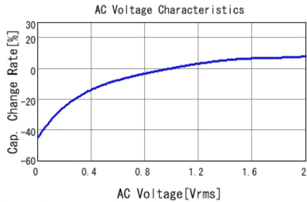
GRM219R61E106KA12 C-AC Voltage capchange, DCOV, 25
