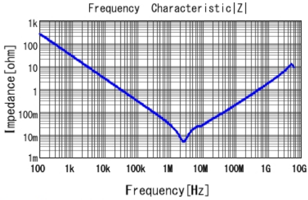
GRM219R61E106KA12 |Z| DCOV, 25degC
