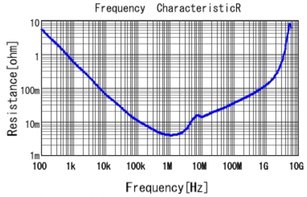
GRM219R61E106KA12 R DCOV, 25degC
