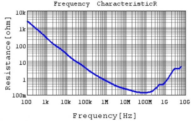
GCM188R72A332KA37 R DC0V, 25degC
