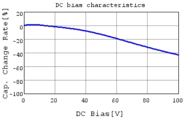
GCM188R72A332KA37 C-DC bias capchange, 25.0c
