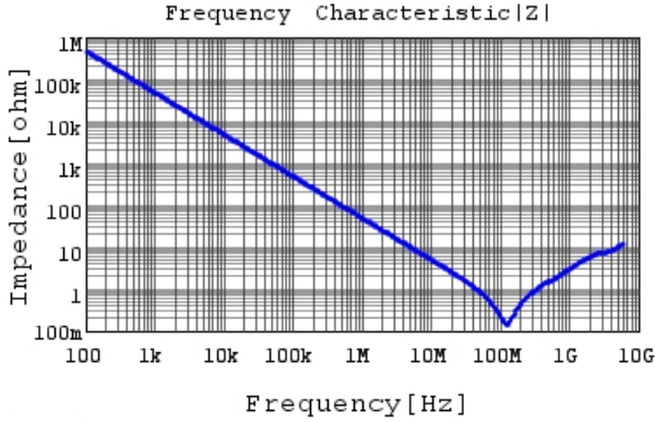
GCM188R72A332KA37 |Z| DC0V, 25degC
