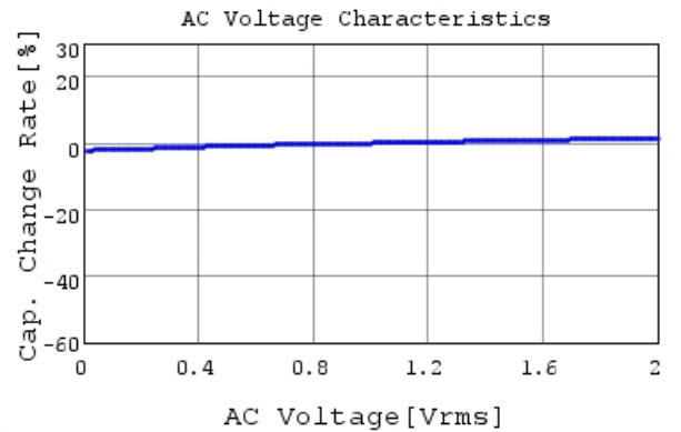
GCM188R72A332KA37 C-AC Voltage capchange, DC
