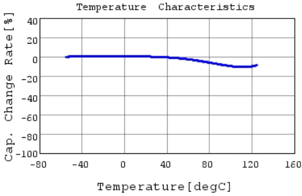
GCM188R72A332KA37 C-Temp. capchange, DC0.0V,
