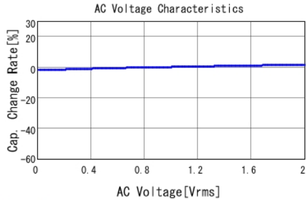
GRM188R71H472MA01 C-AC Voltage capchange, DCOV, 25
