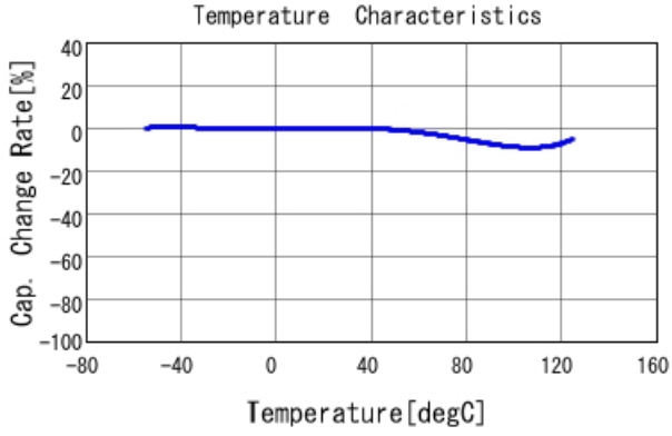
GRM188R71H472MA01 C-Temp. capchange, DC0.0V, AC1.C
