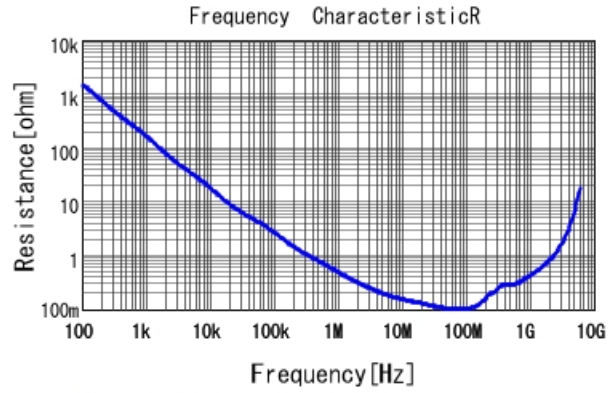
GRM188R71H472MA01 R DCOV, 25degC
