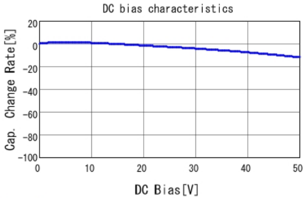
GRM188R71H472MA01 C-DC bias capchange, 25.0degC, A
