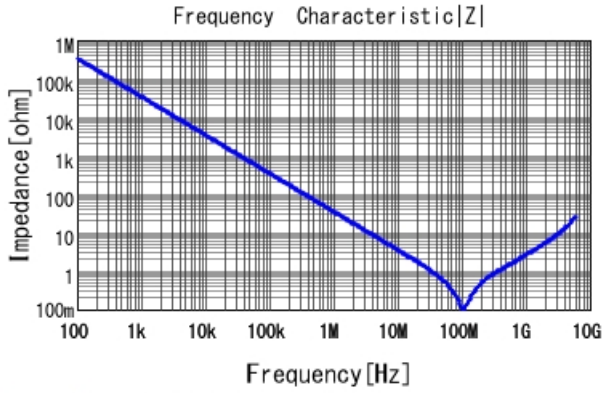
GRM188R71H472MA01 |Z| DCOV, 25degC
