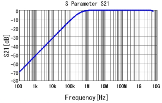
GRM188R71H472MA01 S21 DC0V, 25degC
