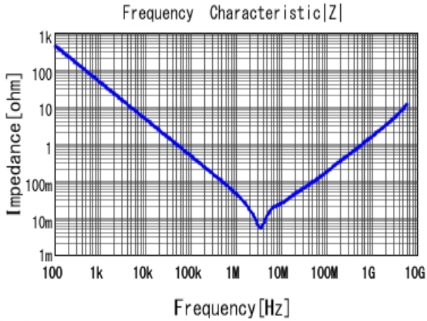
■ GRT188C80J475ME01 |Z| DCOV, 25degC
