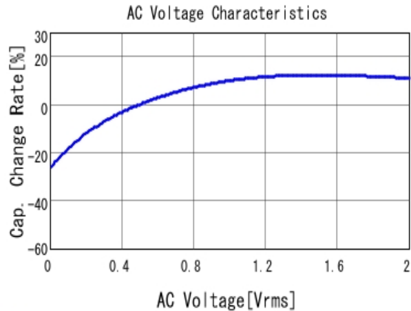
■ GRT188C80J475ME01 C-AC Voltage capchange, DCOV, 25.0d
