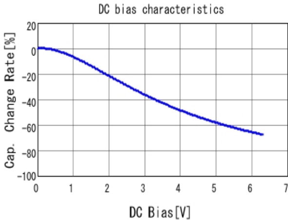
■ GRT188C80J475ME01 C-DC bias capchange, 25.0degC, ACO.
