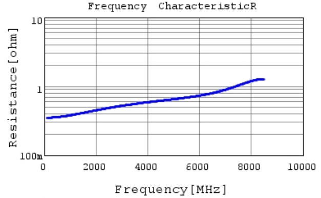
GCM1555C1H1R8BA16 R DCOV,25degC
