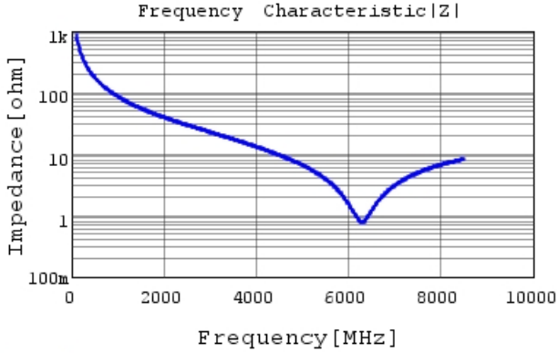
GCM1555C1H1R8BA16 |Z| DCOV,25degC
