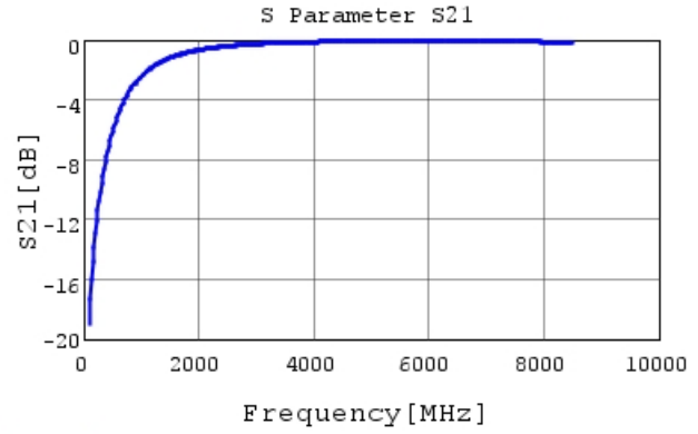
GCM1555C1H1R8BA16 S21 DCOV, 25degC
