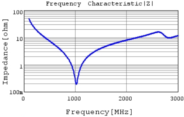
GRM31A5C3A330GW01 |Z| DC0V, 25degC
