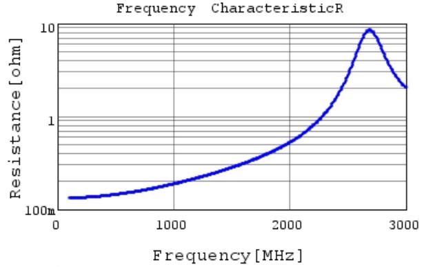
GRM31A5C3A330GW01 R DC0V, 25degC
