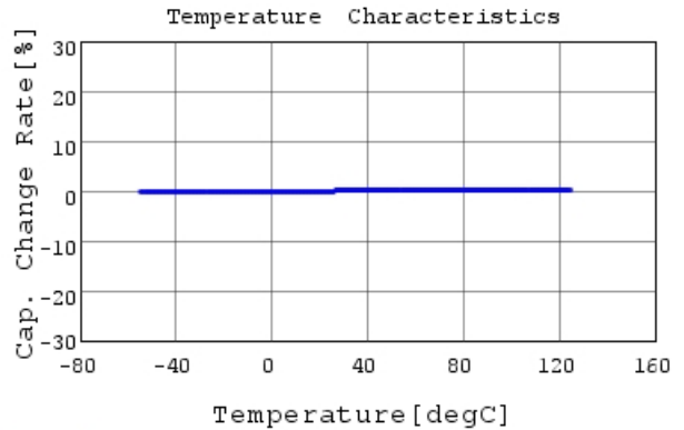
GRM31A5C3A330GW01 C-Temp. capchange, DC0V, 1
