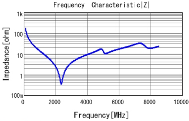
GRM1885C1H9R4CA01 |Z| DCOV, 25degC
