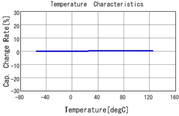
GRM1885C1H9R4CA01 C-Temp. capchange, DCOV, AC1Vrms
