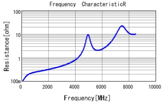
GRM1885C1H9R4CA01 R DCOV, 25degC
