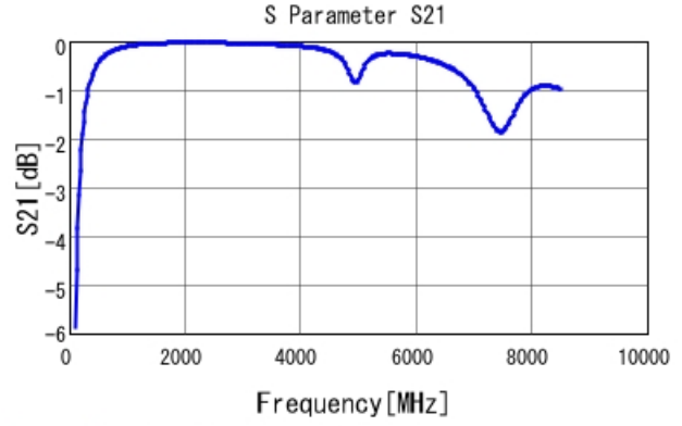
GRM1885C1H9R4CA01 S21 DCOV, 25degC
