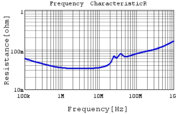
RCER72A334K1K1H03B R DCOV, 25degC
