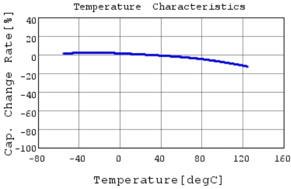
RCER72A334K1K1H03B C-Temp. capchange, DC0.0V
