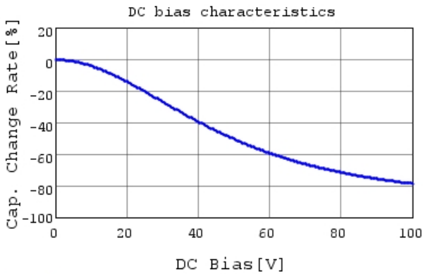
RCER72A334K1K1H03B C-DC bias capchange, 25.0
