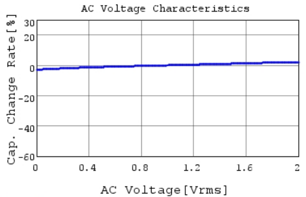
RCER72A334K1K1H03B C-AC Voltage capchange, I
