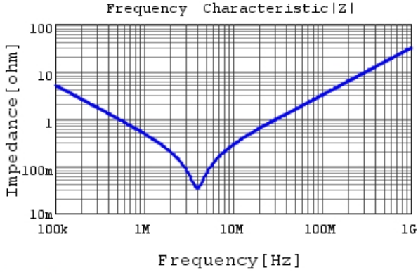
RCER72A334K1K1H03B |Z| DCOV, 25degC
