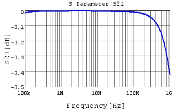
RCER72A334K1K1H03B S21 DC0V, 25degC
