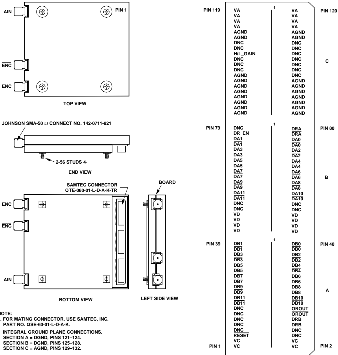
Figure 5. Pin Configuration
