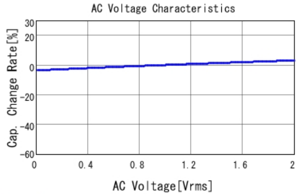
GCJ21BR71E334MA01 C-AC Voltage capchange, DCOV, 25
