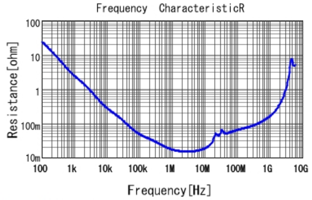
GCJ21BR71E334MA01 R DCOV, 25degC
