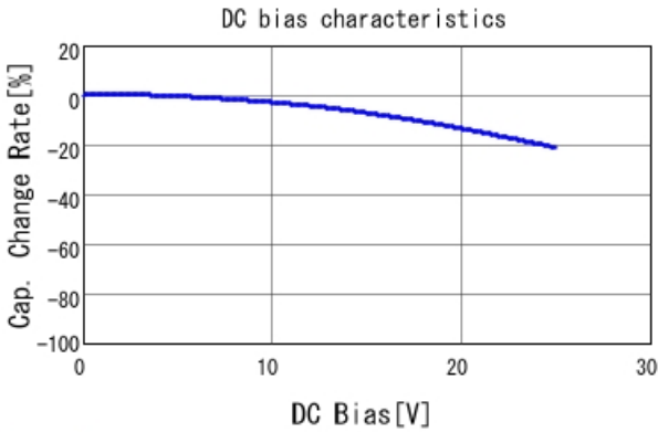
GCJ21BR71E334MA01 C-DC bias capchange, 25.0degC, A
