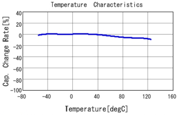
GCJ21BR71E334MA01 C-Temp. capchange, DC0.0V, AC1.C
