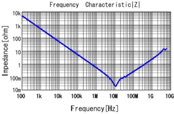
GCJ21BR71E334MA01 |Z| DCOV, 25degC
