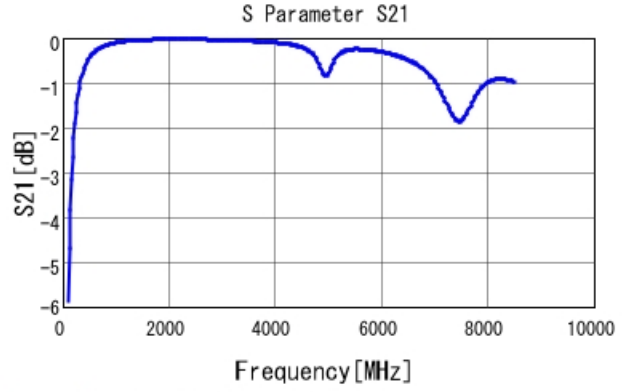
GRM1885C1H9R4BA01 S21 DCOV, 25degC
