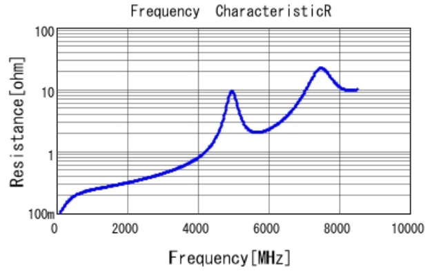
GRM1885C1H9R4BA01 R DCOV, 25degC
