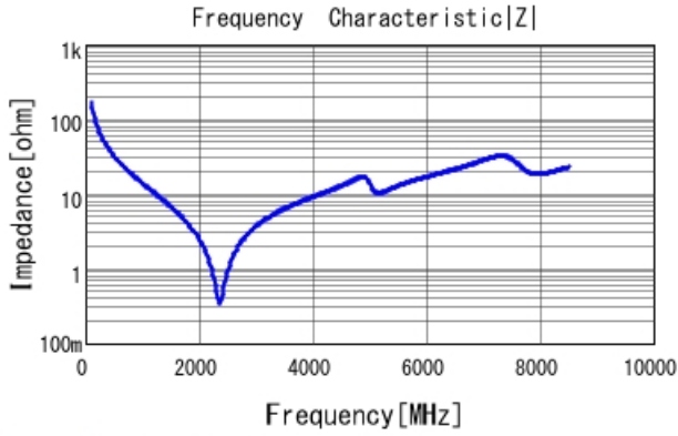
GRM1885C1H9R4BA01 |Z| DCOV, 25degC
