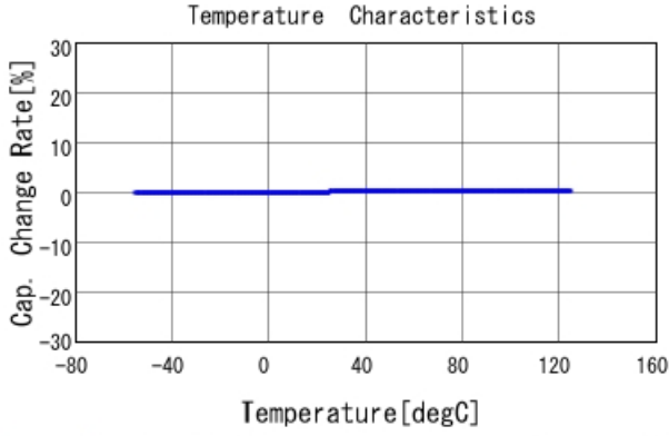
GRM1885C1H9R4BA01 C-Temp. capchange, DCOV, AC1Vrms
