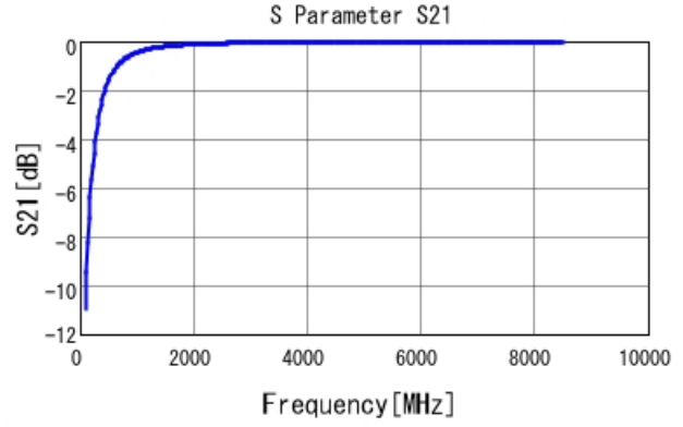
GRM0225C1E4R7BA03 S21 DC0V, 25degC
