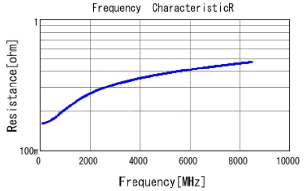
GRM0225C1E4R7BA03 R DCOV, 25degC
