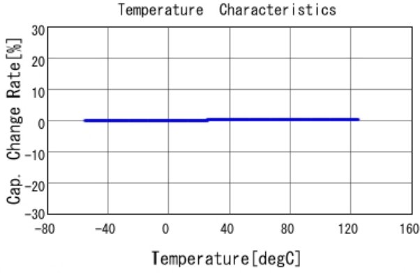
GRM0225C1E4R7BA03 C-Temp. capchange, DC0V, AC1Vrms
