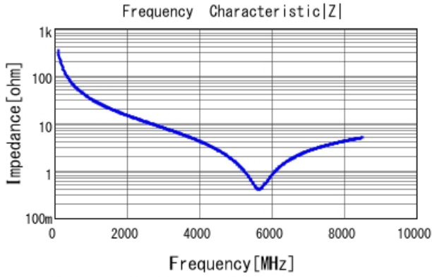
GRM0225C1E4R7BA03 |Z| DCOV, 25degC
