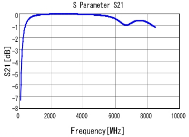
■ GRM1555C2A7R6DA01 S21 DCOV, 25degC
