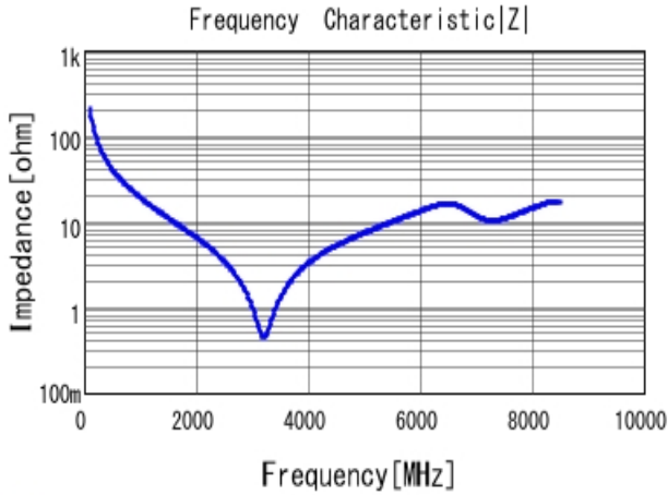
■ GRM1555C2A7R6DA01 |Z| DCOV, 25degC
