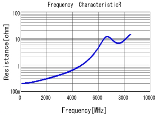
■ GRM1555C2A7R6DA01 R DCOV, 25degC
