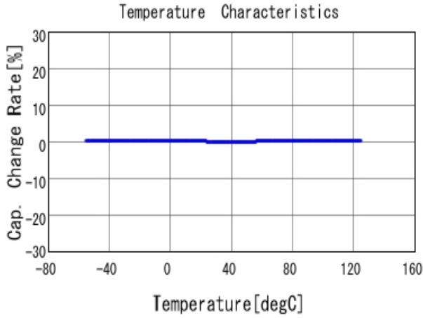
■ GRM1555C2A7R6DA01 C-Temp. capchange, DCOV, AC1Vrms
