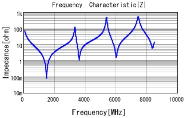
GQM22M5C2H220GB01 |Z| DCOV, 25degC
