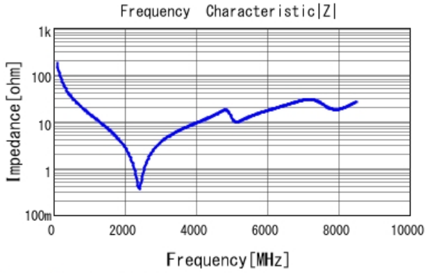
GRM1885C1H9R0WA01 |Z| DCOV, 25degC
