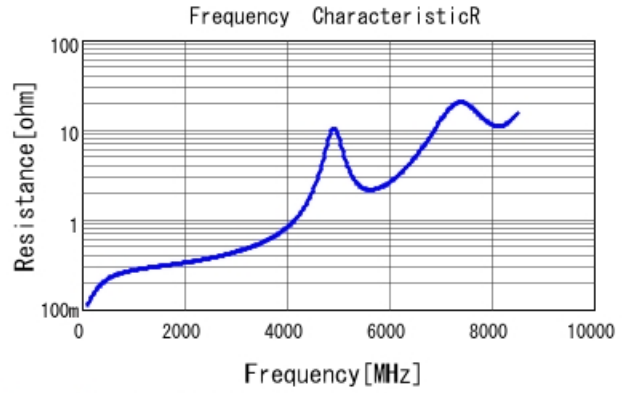
GRM1885C1H9R0WA01 R DCOV, 25degC
