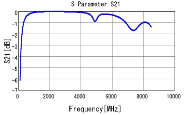
GRM1885C1H9R0WA01 S21 DCOV, 25degC
